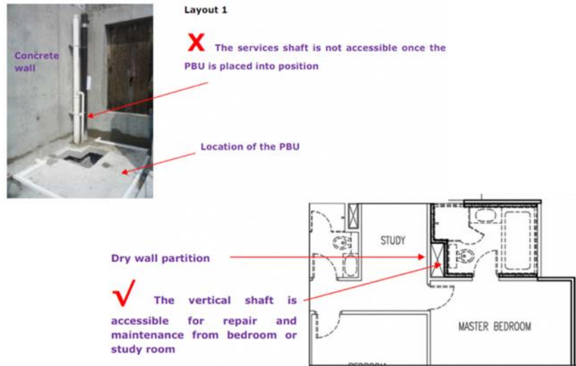
Figure 1: Sample layouts with different positions of vertical soil stack (or vertical shaft).
